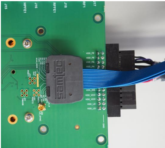
Figure 19: Connect IO Cable to P1 on Evaluation Board
