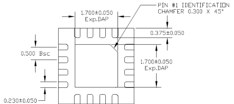
BOTTOM VIEW
